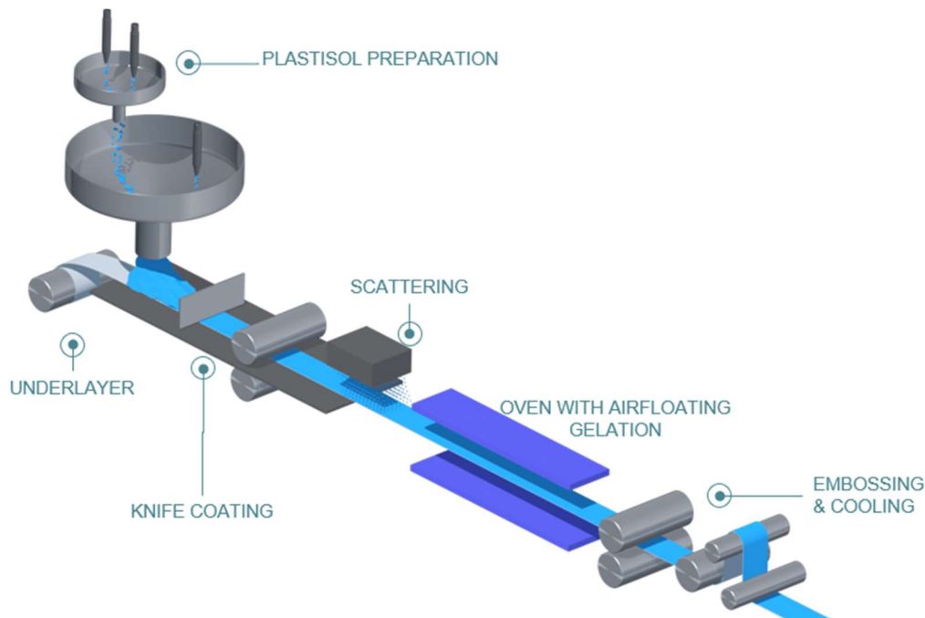
Figure 1: Coating process
